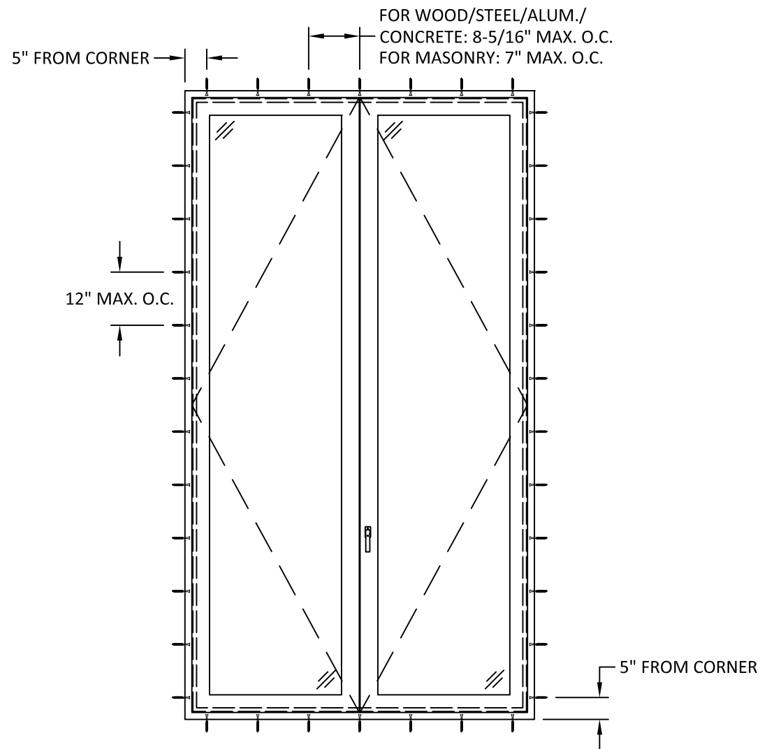
ANCHOR LAYOUT FRENCH CASEMENT
