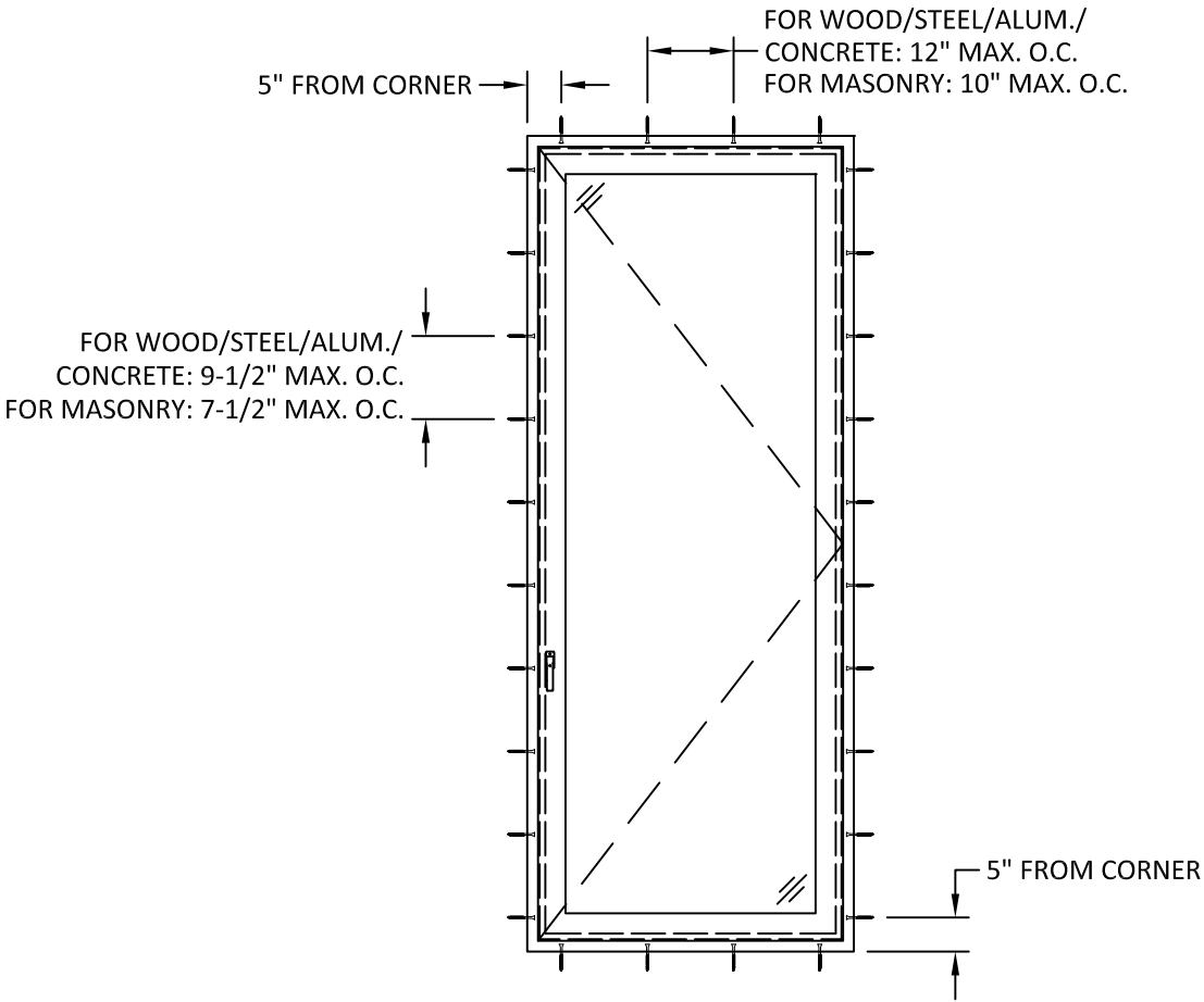
ANCHOR LAYOUT SINGLE CASEMENT
