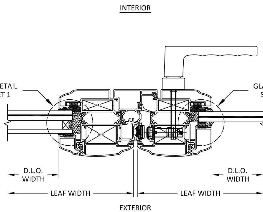
D 5 HORIZONTAL SECTION MEETING STILE
